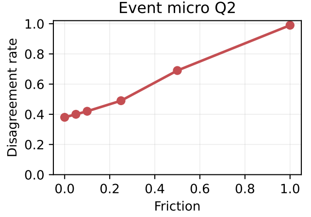
Figure 3: Appendix-promoted event-micro robustness view. In the main forecasting-native benchmark, disagreement between forecast-side and deployed-side selection is lowest at zero and very low friction and increases as switching frictions rise.
