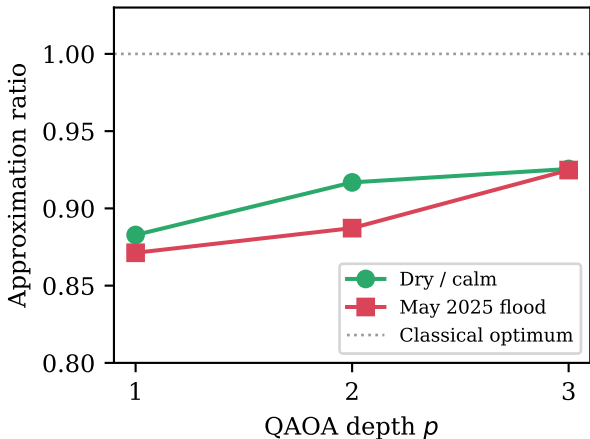
QAOA convergence (INTERP warm start)
