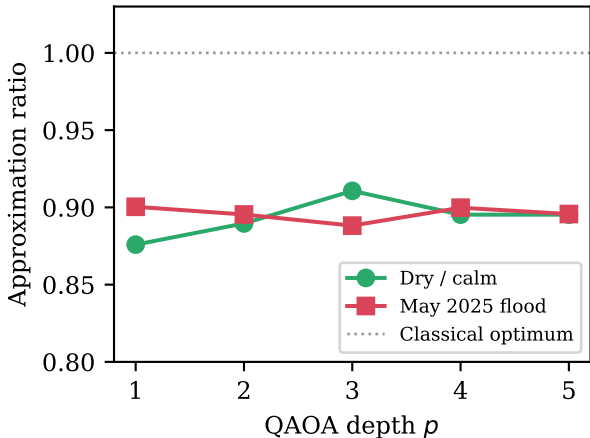
QAOA depth study (five-seed mean)
