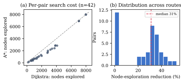
FIGURE 14. (a) Per-pair search cost; points below the diagonal indicate A^* explored fewer nodes. (b) Distribution of per-pair node-exploration reduction, median 31.1%.
