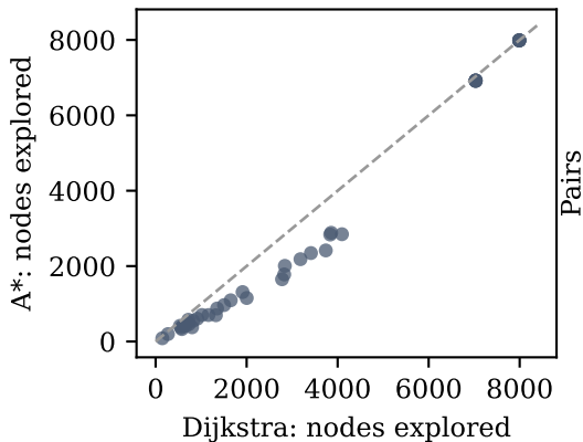
(a) Per-pair search cost (n=42)
