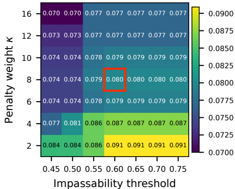
(a) Mean exposure (common 20 pairs)
