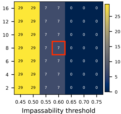
(c) Severed pairs (of 49)
