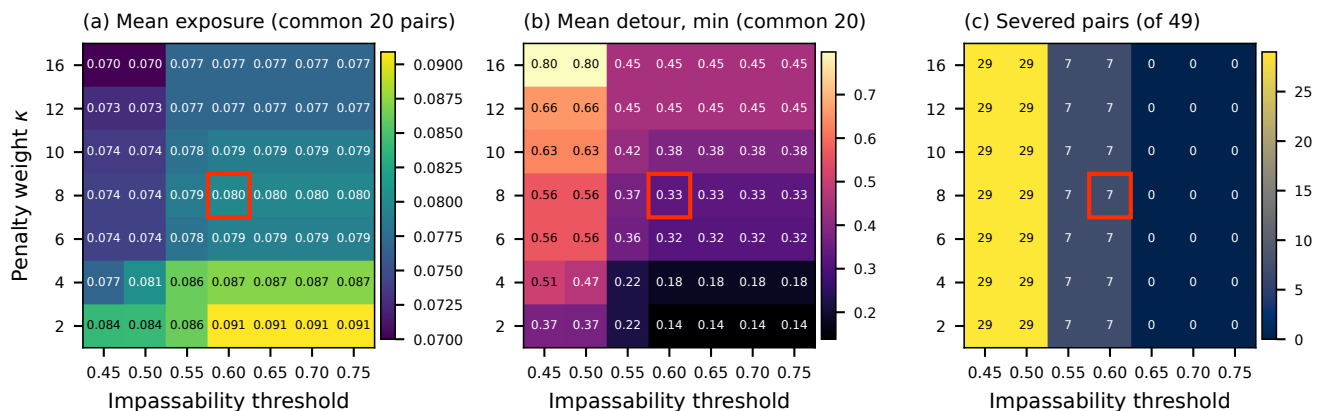
FIGURE 13. Sensitivity of the routing outcome to the penalty weight \kappa and impassability threshold \tau at T = 0.70 . (a) Mean route exposure and (b) mean detour, both over the 20 pairs routable in every cell of the sweep so that cells are compared like with like; (c) severed pairs, over all 49. Vertical banding shows the outcome depends on \tau far more than on \kappa ; the red box marks the operating point.
