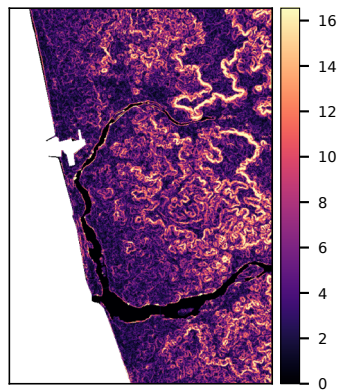
HAND (m)
