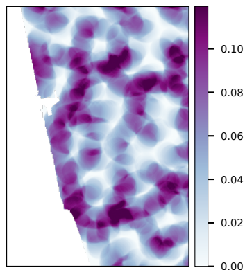
Drainage density (-)
