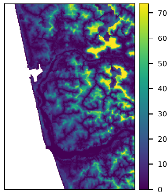
Drainage density (-)
