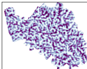
Drainage density (-)
