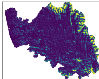
HAND (m)
