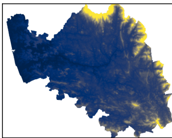
Elevation (m)
