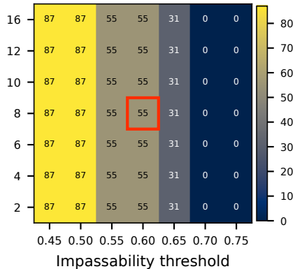
(c) Severed pairs (of 247)
