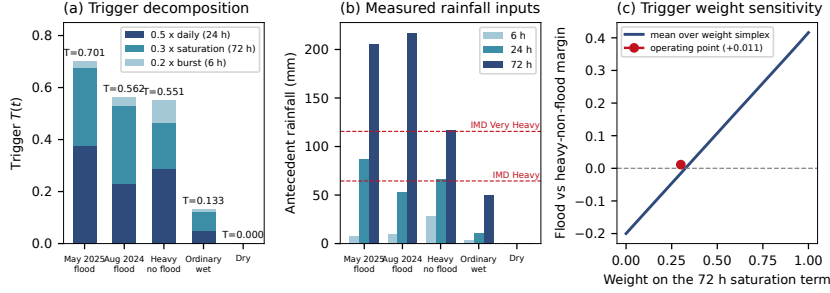
Figure 10: (a) Decomposition of T(t) into its three weighted terms. (b) The measured rainfall inputs. The two documented floods exceeded 200 mm of 72-hour antecedent rainfall; the heavy-rain non-flood day reaches only 116.8 mm despite the largest 6-hour burst in the set, identifying catchment saturation as the discriminating variable. (c) Mean adversarial margin across the weight simplex as a function of the saturation weight, at \theta_{\text{sat}} = 200 mm. The operating point sits almost exactly at the zero crossing.
