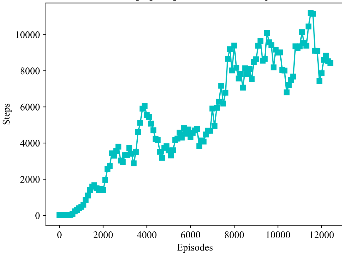
Steps per episode over training
