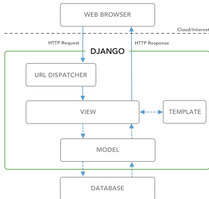
Django Architecture
