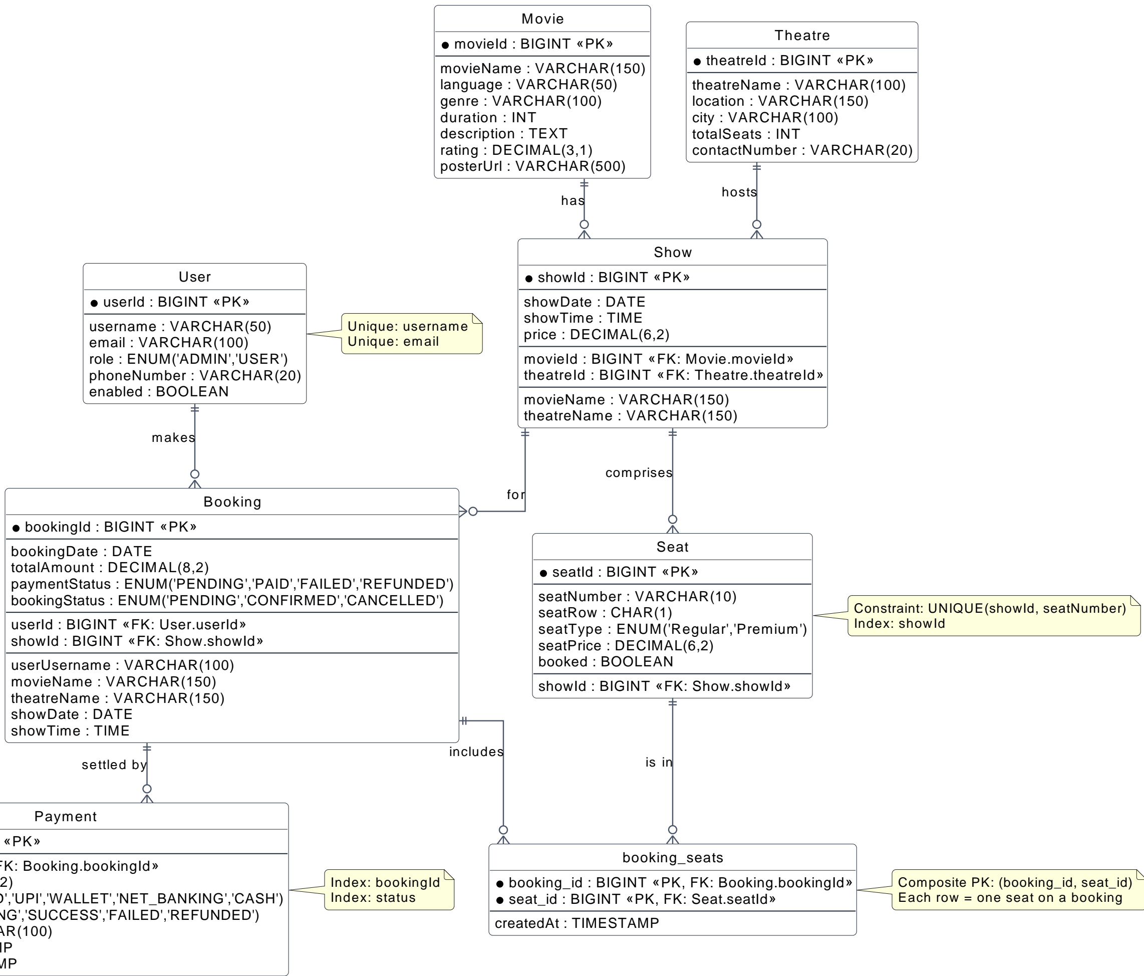
Movie Ticket Booking ER Diagram
