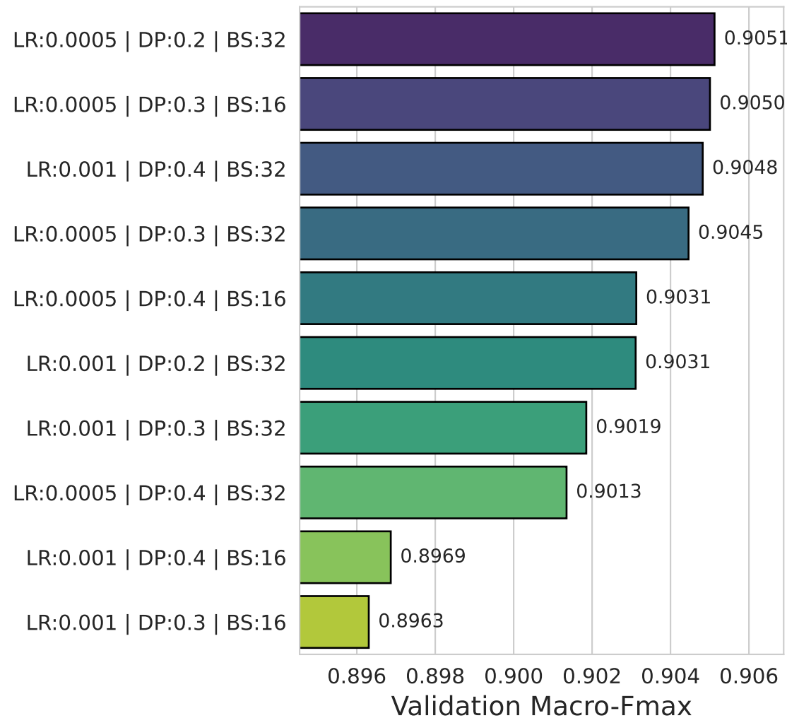
Molecular Function
