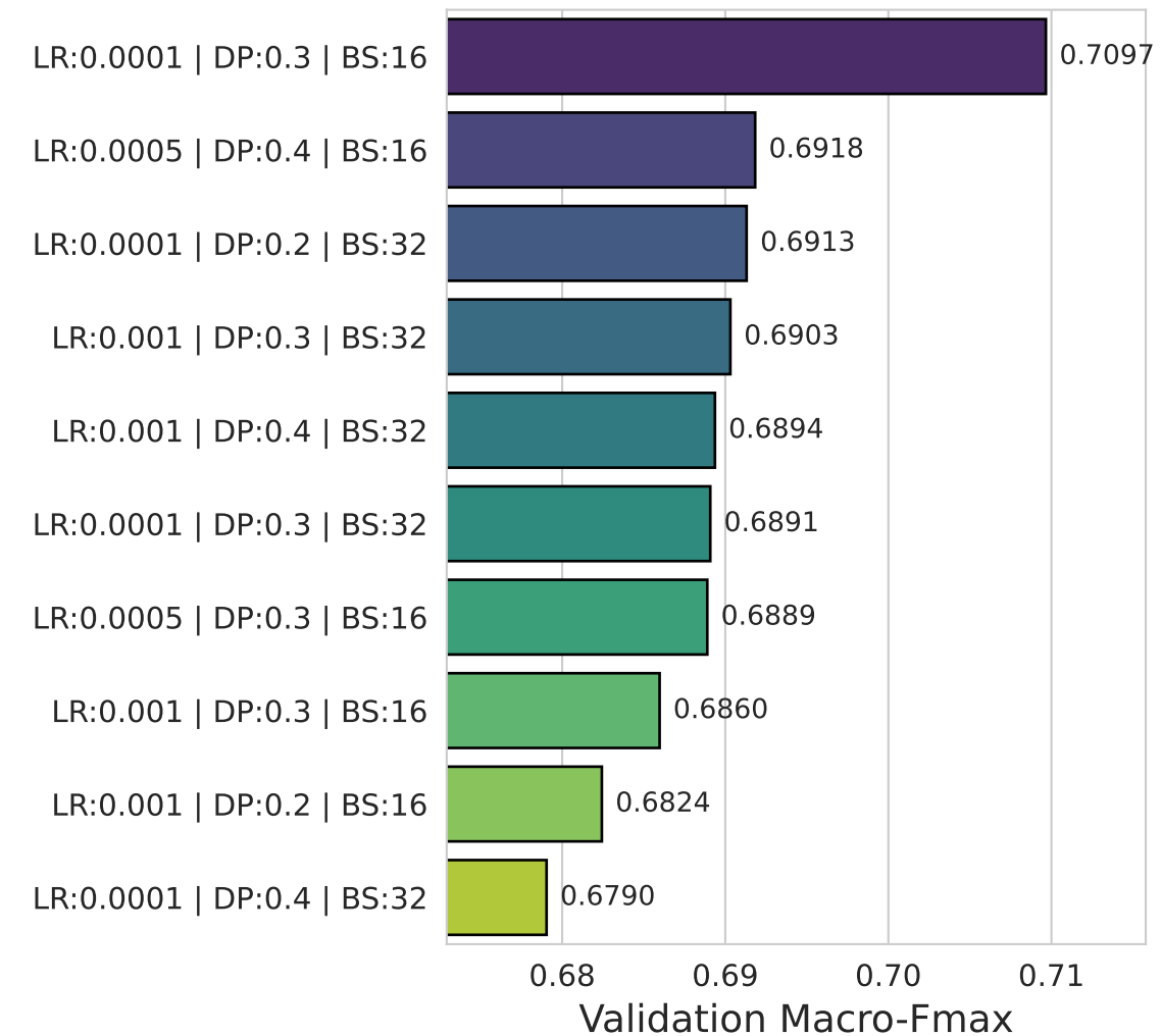
Cellular Component
