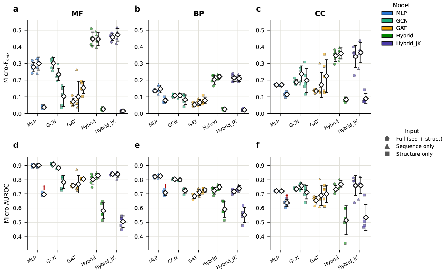
Top row: Micro-F max . Bottom row: Micro-AUROC. Identical layout and colour mapping in both rows — only the metric changes, and the model ranking inverts with it, so neither family alone supports a single 'best model' claim. Error bars show mean \pm s.d. across n = 5 training seeds; points are seeds, open diamonds the mean. † marks the MLP structure-only constant-predictor control (Macro-AUROC 0.500 = chance). Generated by src/plot_arc_ablations.py from ablations/**/test_metrics.json .
