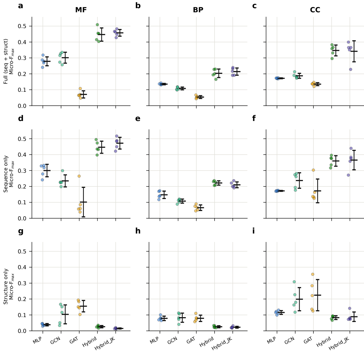
Rows are input modality, columns are GO sub-ontology, and each panel shows the five architectures on a shared y-axis — modality is a facet rather than a marker shape, so no symbol decoding is required. Points are individual seeds; the horizontal bar is the mean with error bars show mean \pm s.d. across n = 5 training seeds. \dagger marks the MLP structure-only constant-predictor control. F_{\max}/S_{\min} favour graph-aware Hybrid/Hybrid_JK. Generated by src/plot_arc_ablations.py from ablations/**test_metrics.json .
