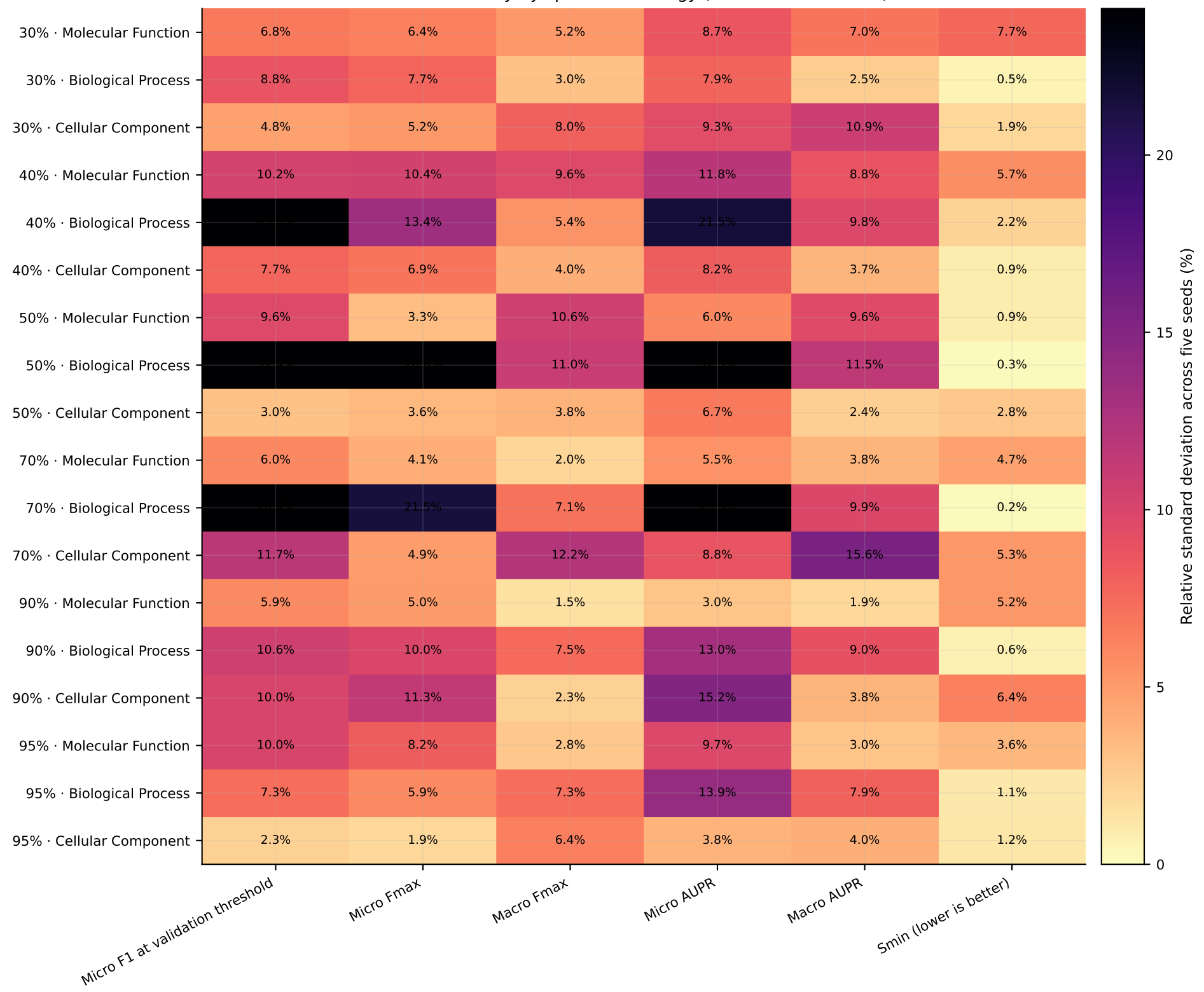
Seed stability by split and ontology (lower is more stable)
