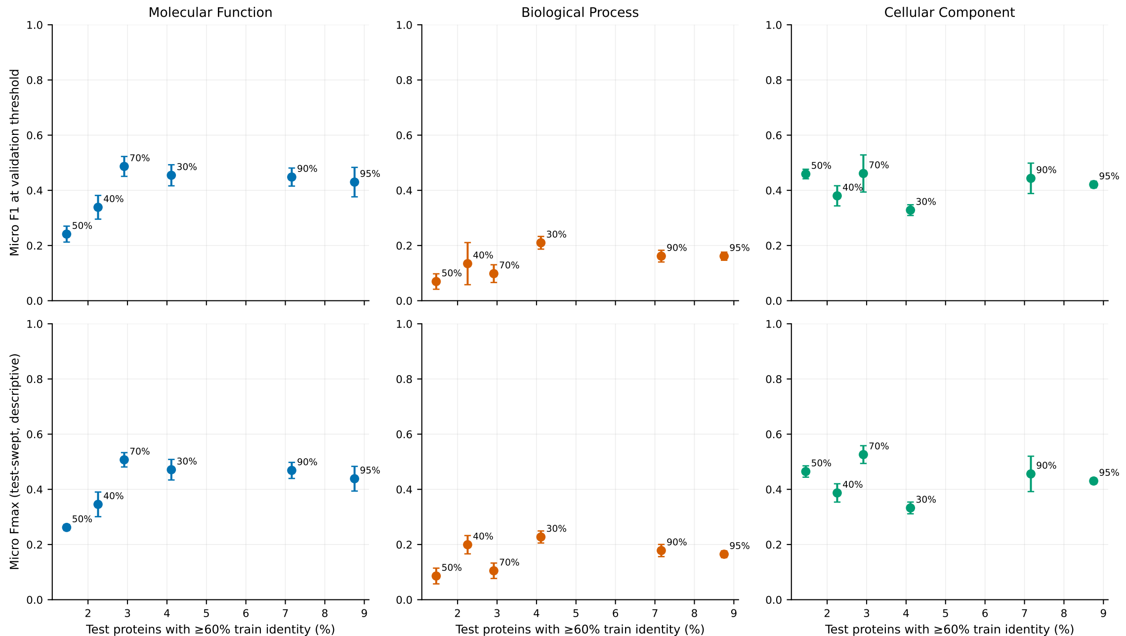
Performance versus measured test-to-train similarity; labels are nominal split thresholds
