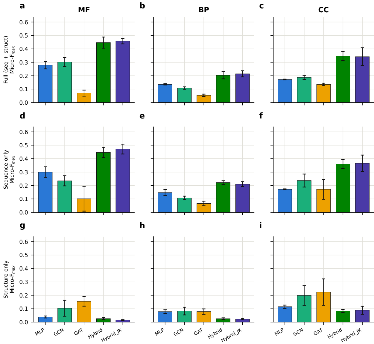
Rows are input modalities and columns are ontologies. Bars show the mean with mean \pm SD across five seeds; higher is better. Bars are grouped/faceted, not stacked, because model scores are not additive. F_{max}/S_{min} favour graph-aware Hybrid/Hybrid_JK.
