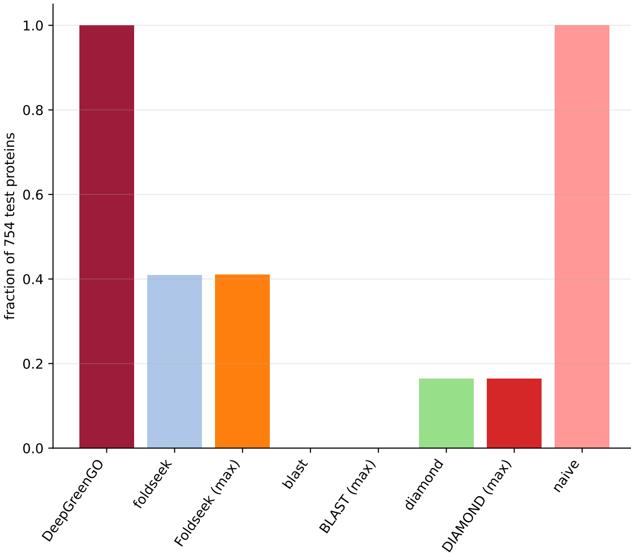
Molecular Function
