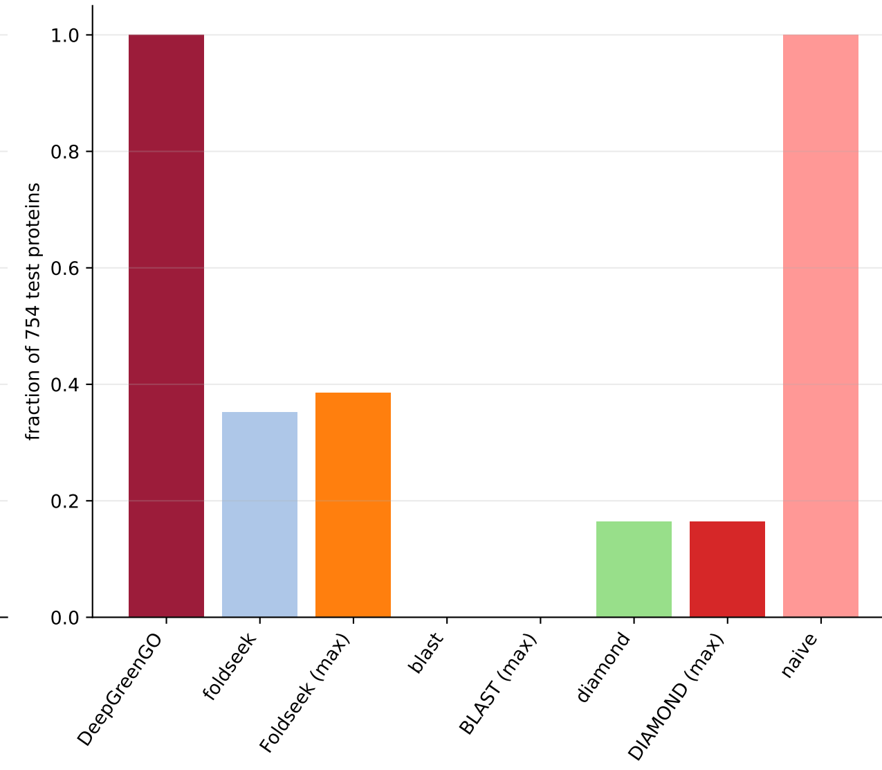
Biological Process
