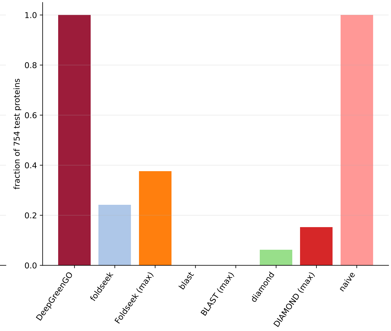
Cellular Component
