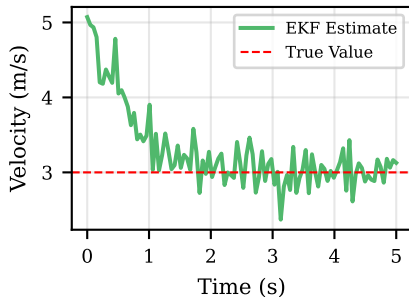
Velocity Convergence
