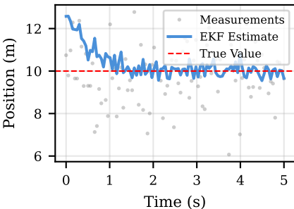
Position Convergence
