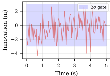
EKF Innovation
