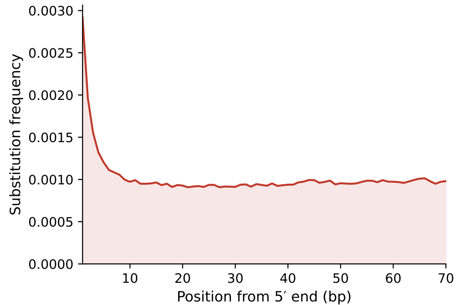
C→T (5' end)
