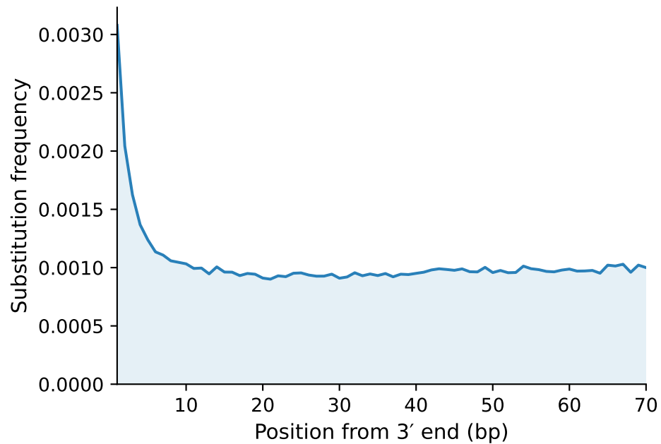
G→A (3' end)
