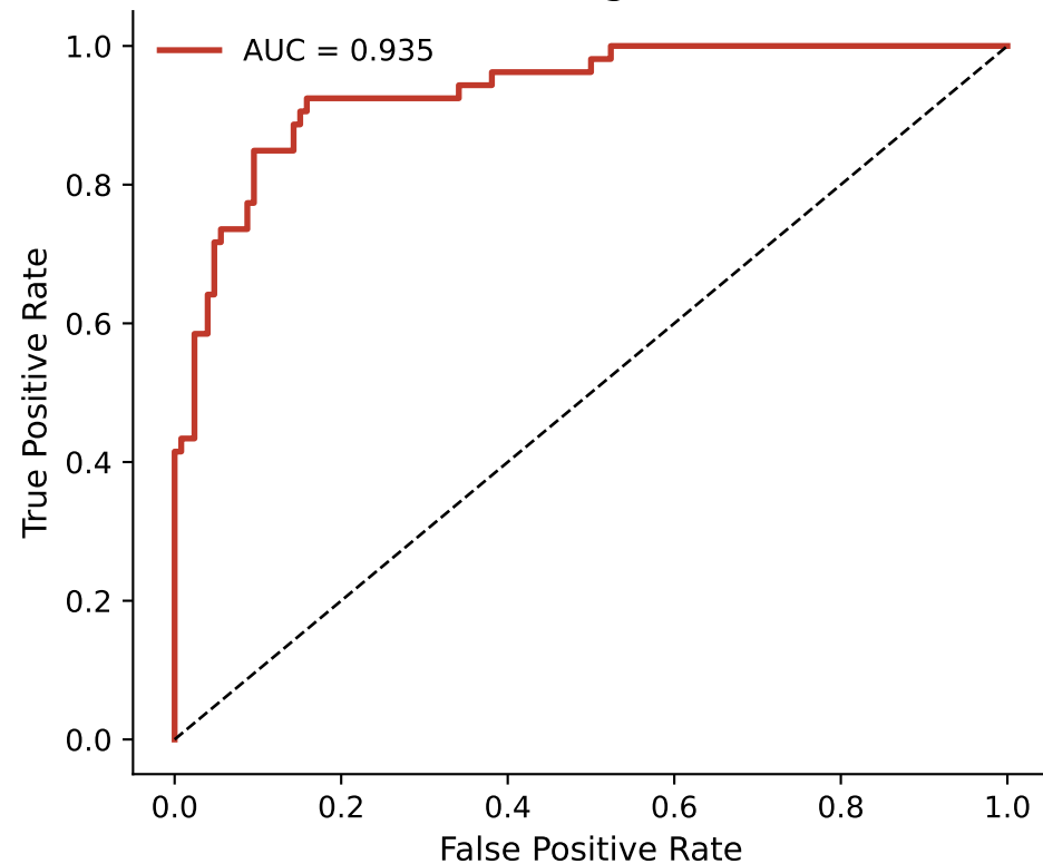
ROC — Pathogen vs Host
