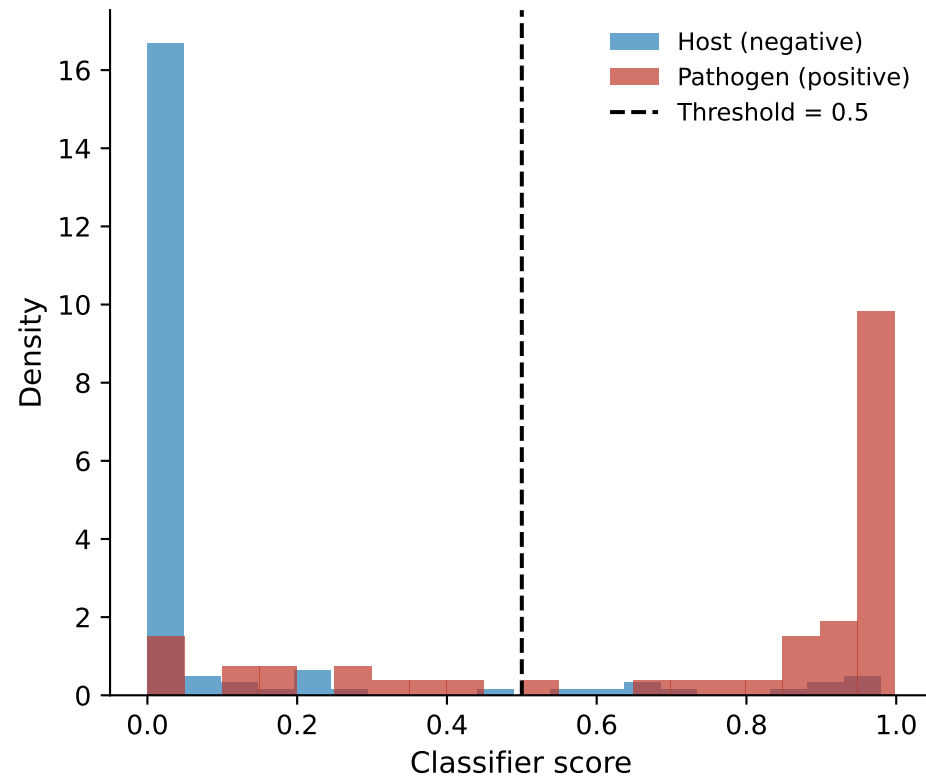
Score distribution (validation set)
