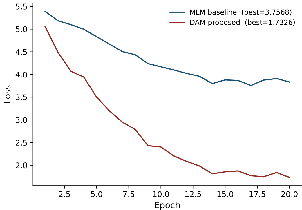
Validation Loss
