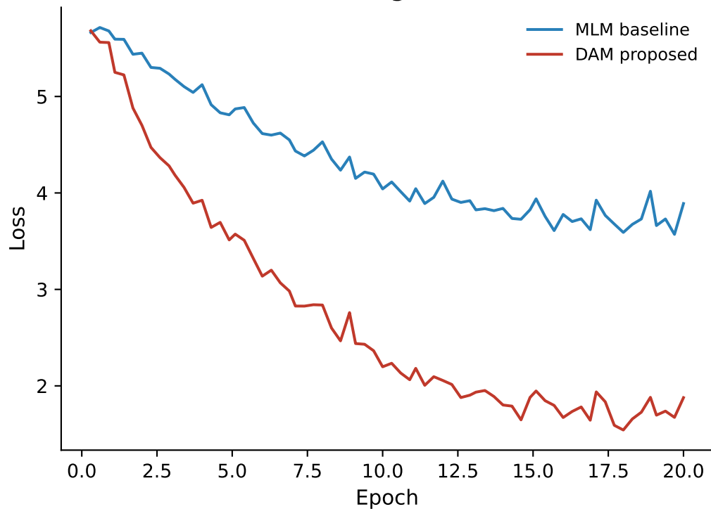
Training Loss
