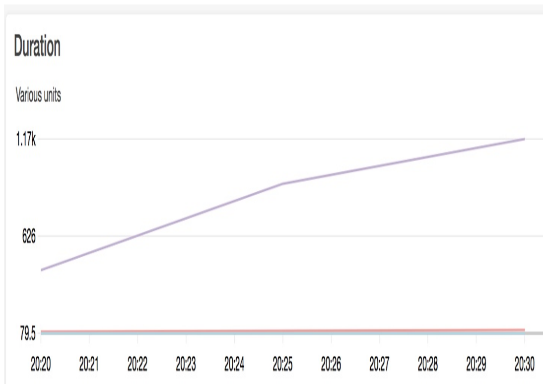
Figure 13-3. Lambda duration
