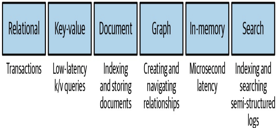
Figure 15-4. Amazon databases
