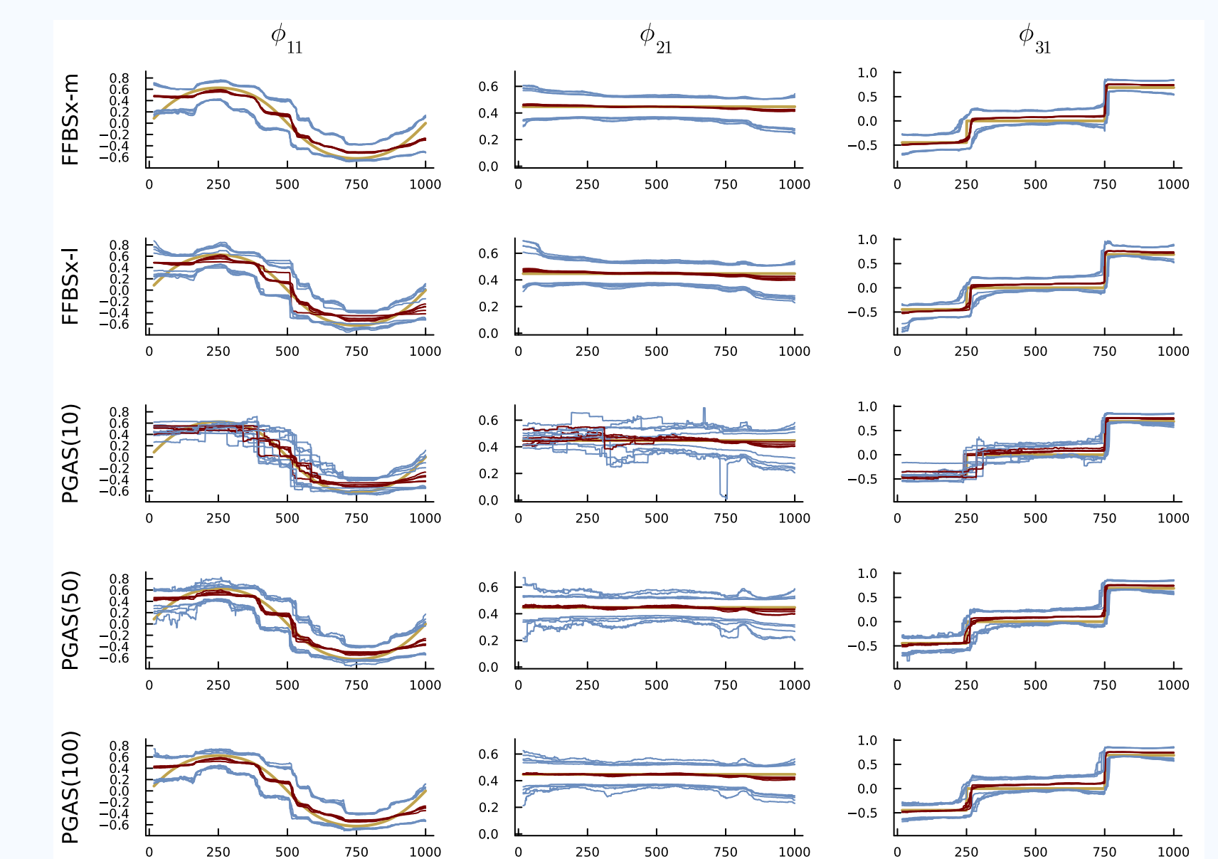
TV-SAR(1,1) (4,12) : Posterior medians (red) and 95% credible bands (blue) from five independent runs.
