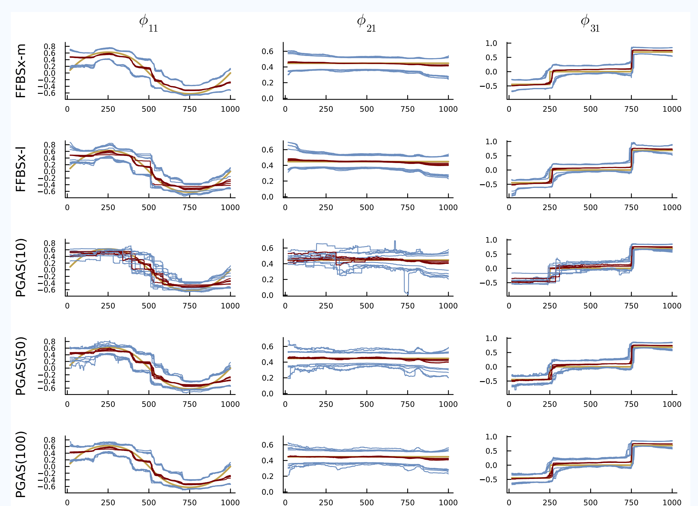
TV-SAR(1,1) 4,12 : Posterior medians (red) and 95% credible bands (blue) from five independent runs.
