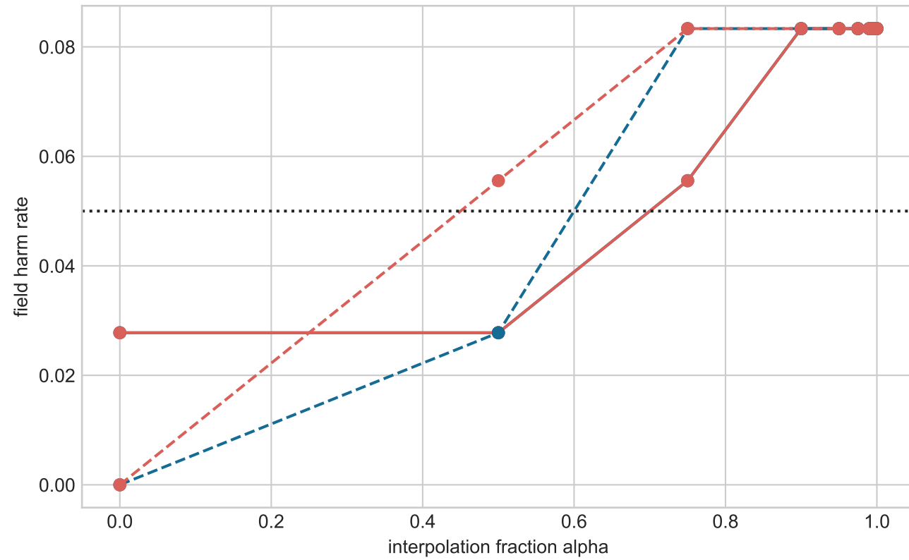
tail-risk gate
