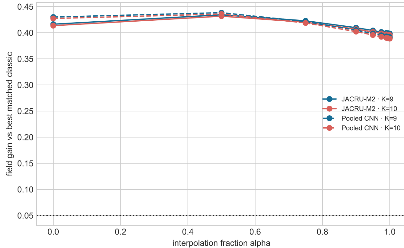
tail-risk gate
