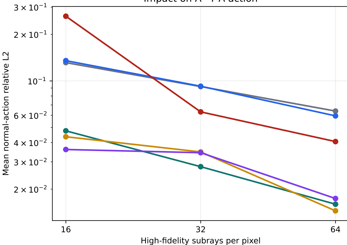
Impact on A^T A action
