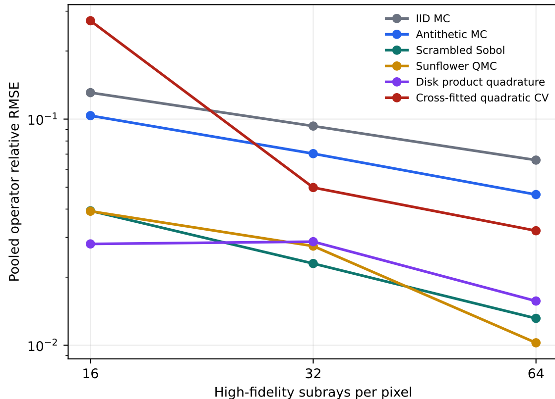
Impact on A^T A action
