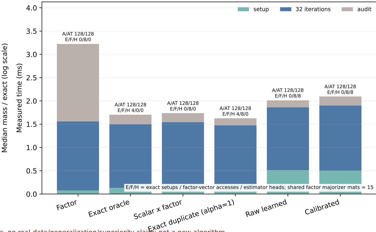
D. Cost/call ledger (single-run timing; not speed evidence)
