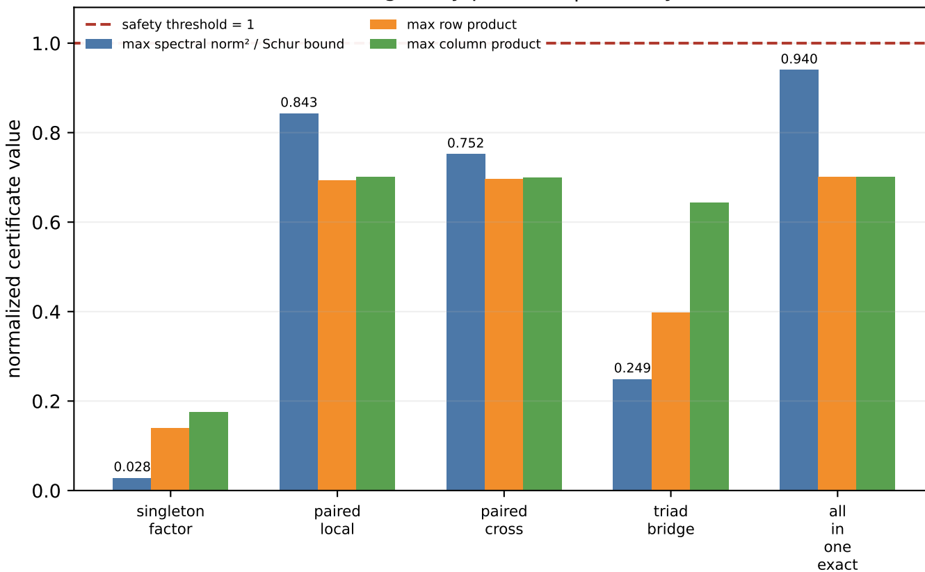
Certificate margins by partition | 0 safety violations
