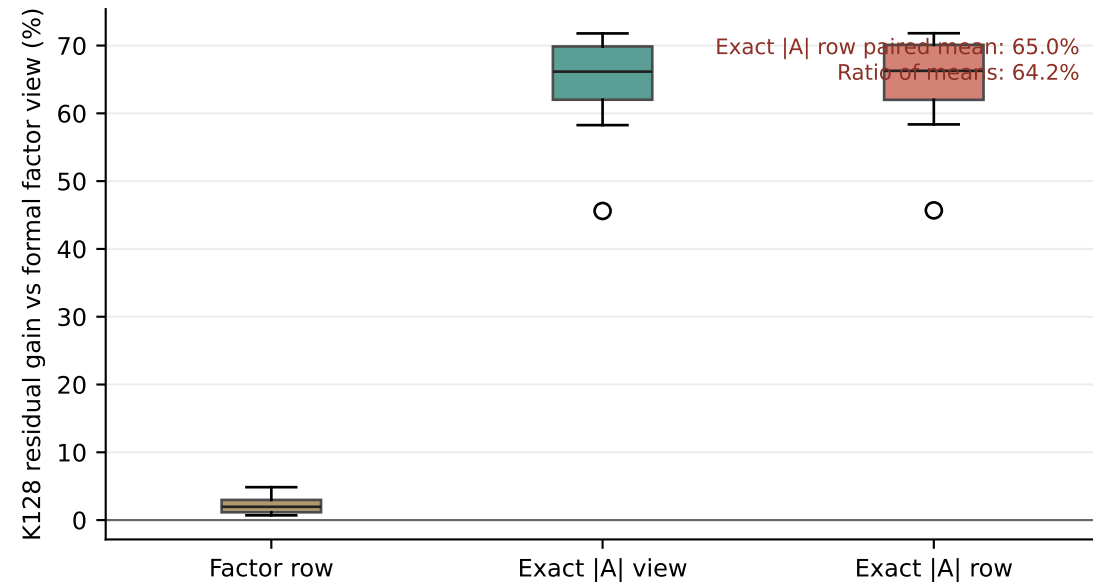
C 2 replicate clusters x 8 shared morphologies (not IID)
