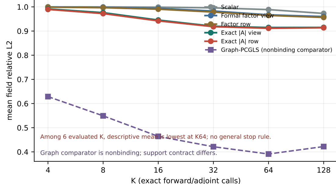
D Exact-to-factor tightness and explicitly labeled slack
