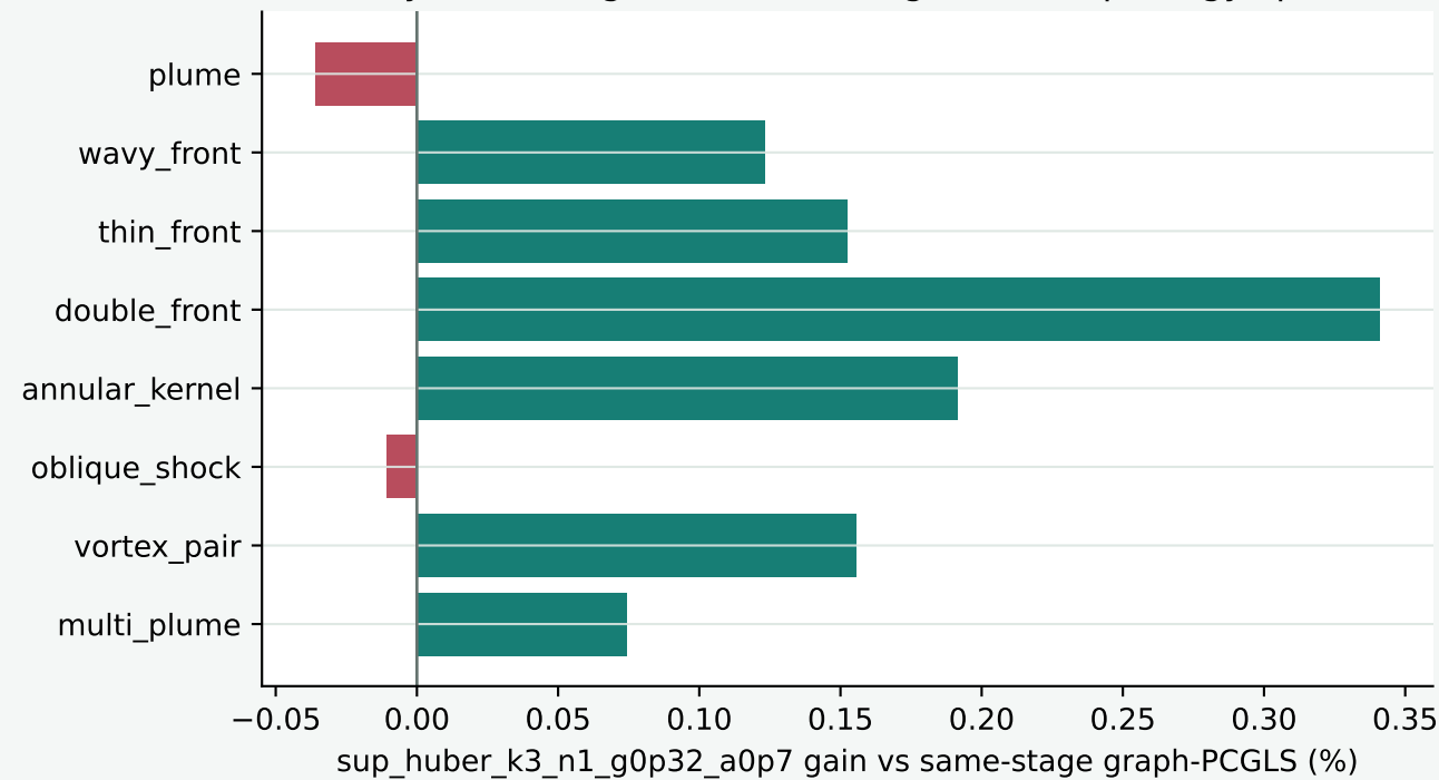
C Tiny same-stage mechanism signal is morphology-specific
