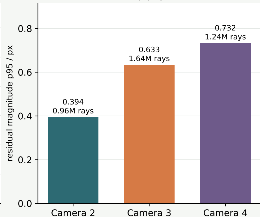
Tail residual by physical camera
