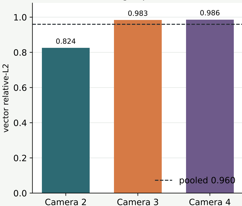
Held-out image-space mismatch
