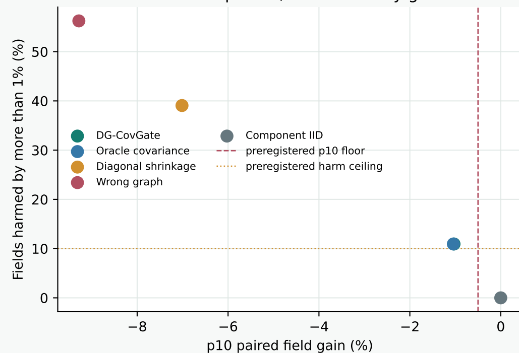
C The mean improves, but the safety gate fails
