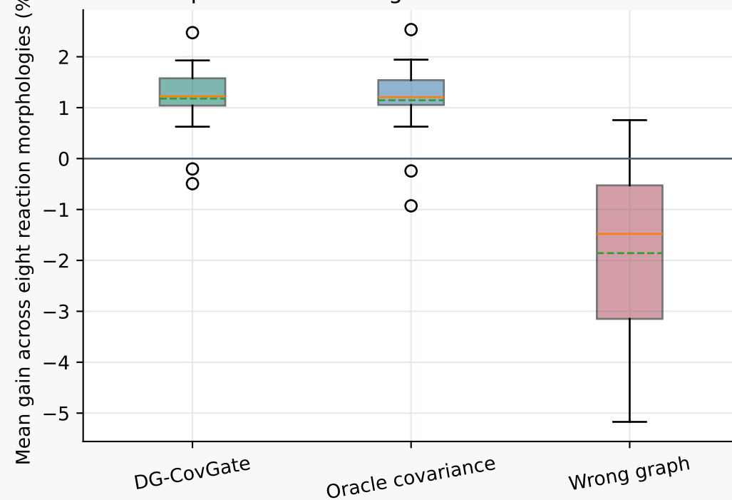
D Replicate-clustered gain across 16 fresh seeds
