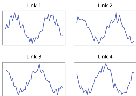
Traffic Flow Sequences X_t
