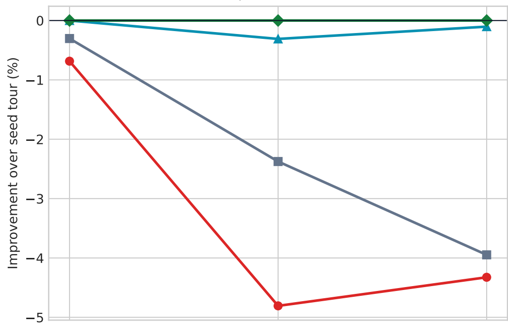
TSP100, 2-opt seed route
