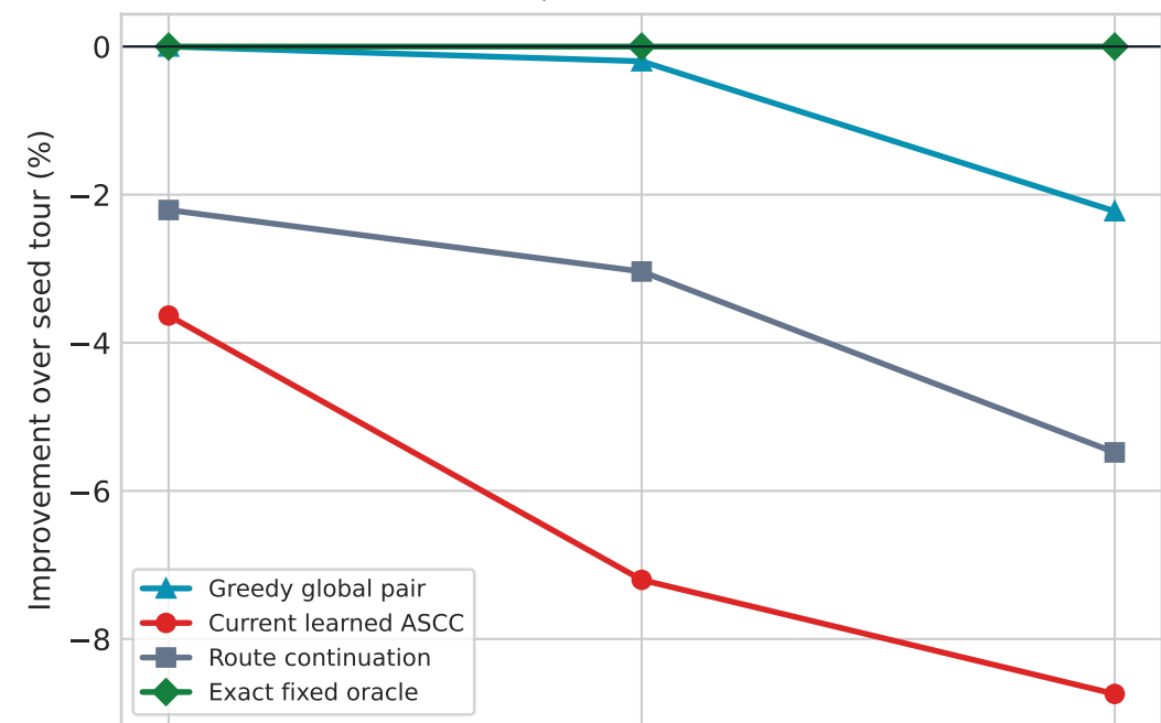
TSP50, 2-opt seed route
