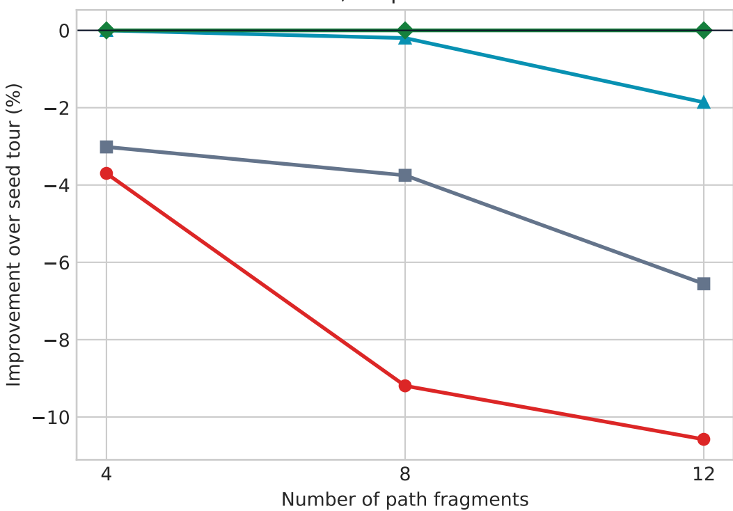
TSP50, 2-opt seed route
