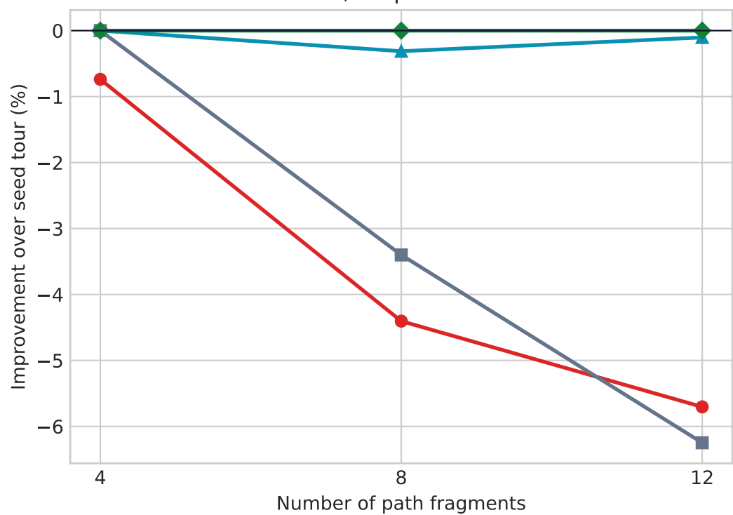
TSP100, 2-opt seed route
