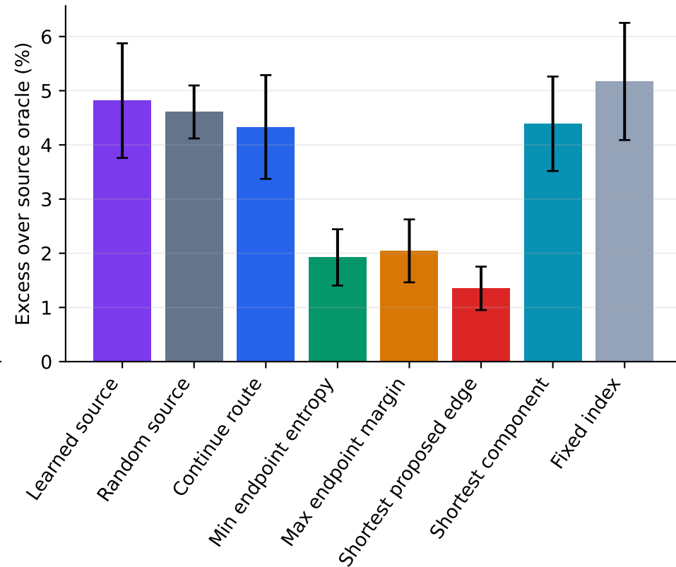
B. Current source policies leave regret
