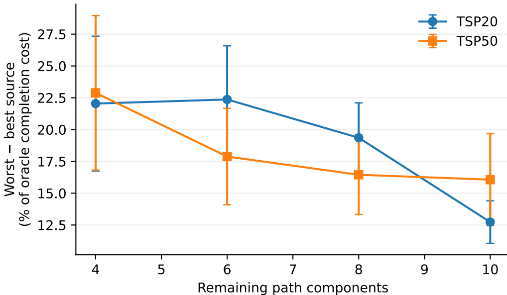
A. Source choice has nonzero opportunity
