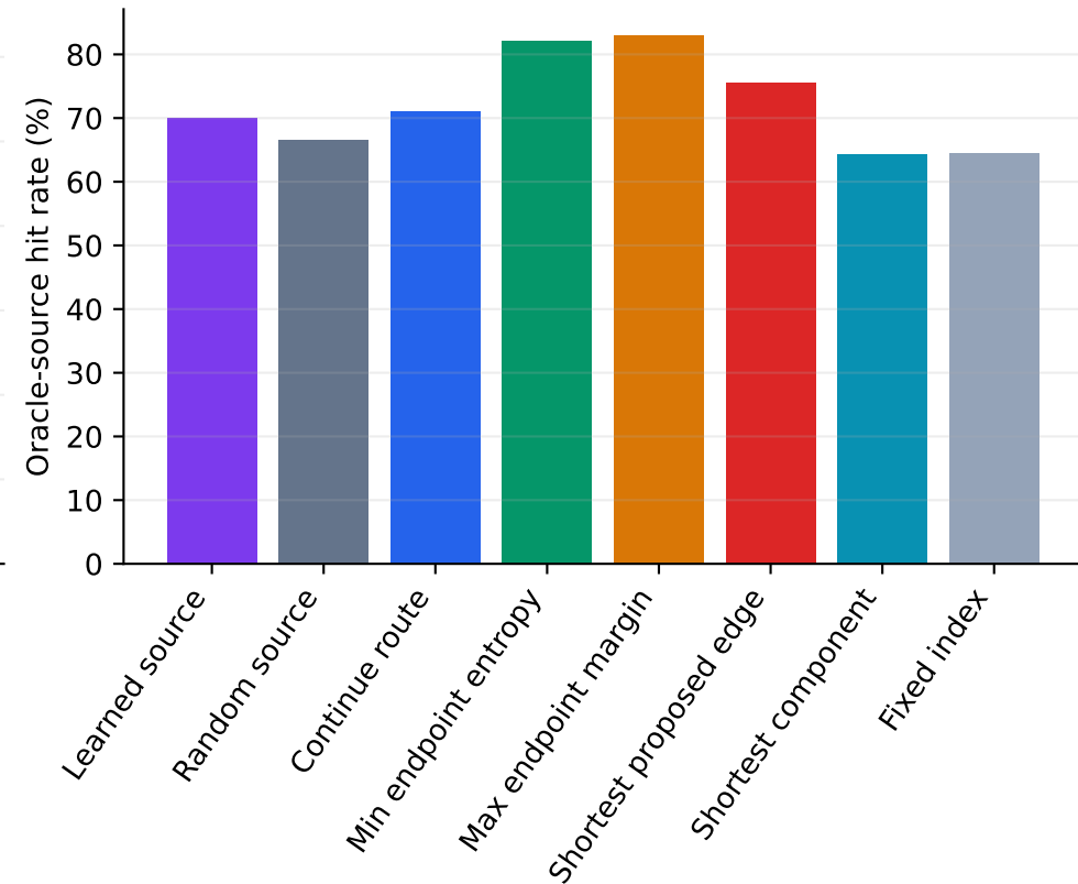
C. How often each policy selects an oracle source
