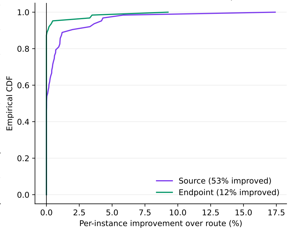
C. TSP50, one intervention at 30 components
