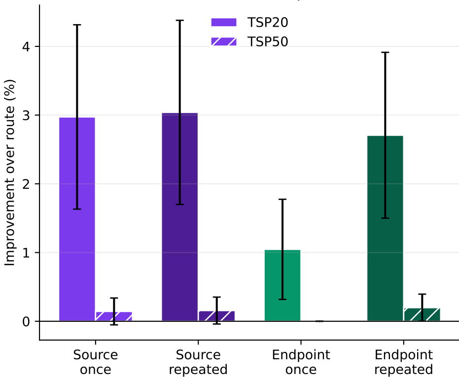
A. Perfect rollout values can improve the final tour
