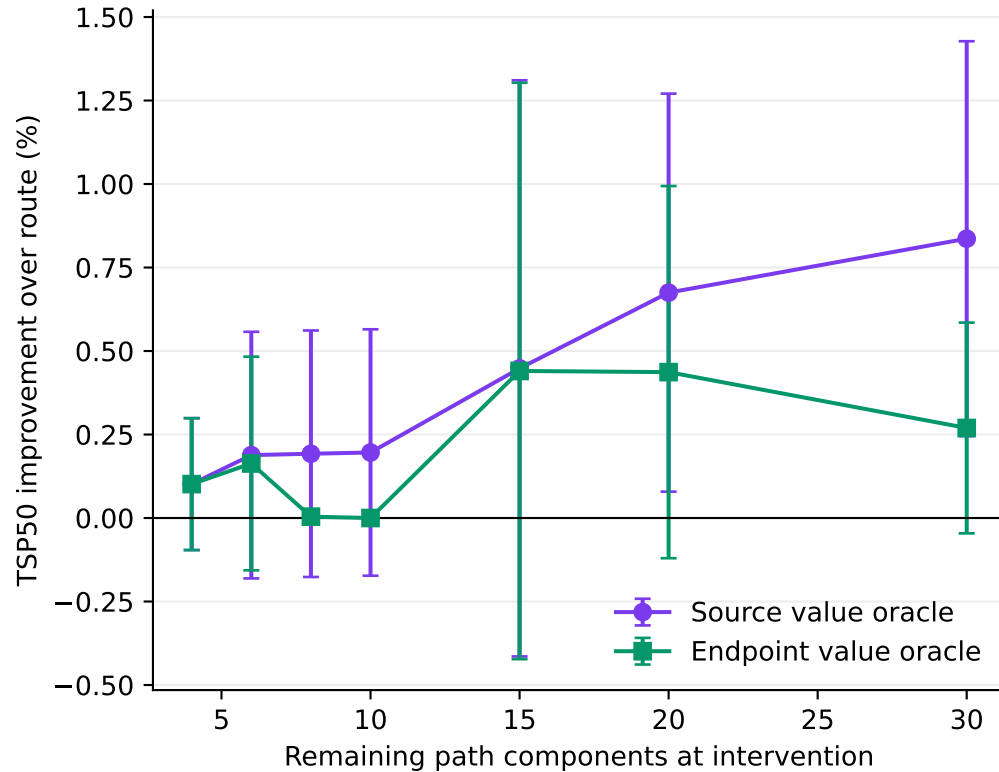
B. Earlier source decisions contain more value
