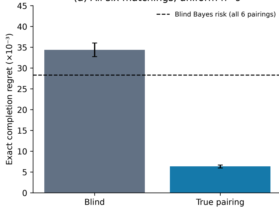
(a) All six matchings, uniform n=9
