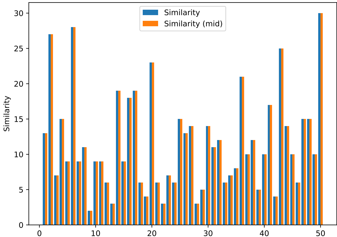
Similarity vs Similarity with mid point
