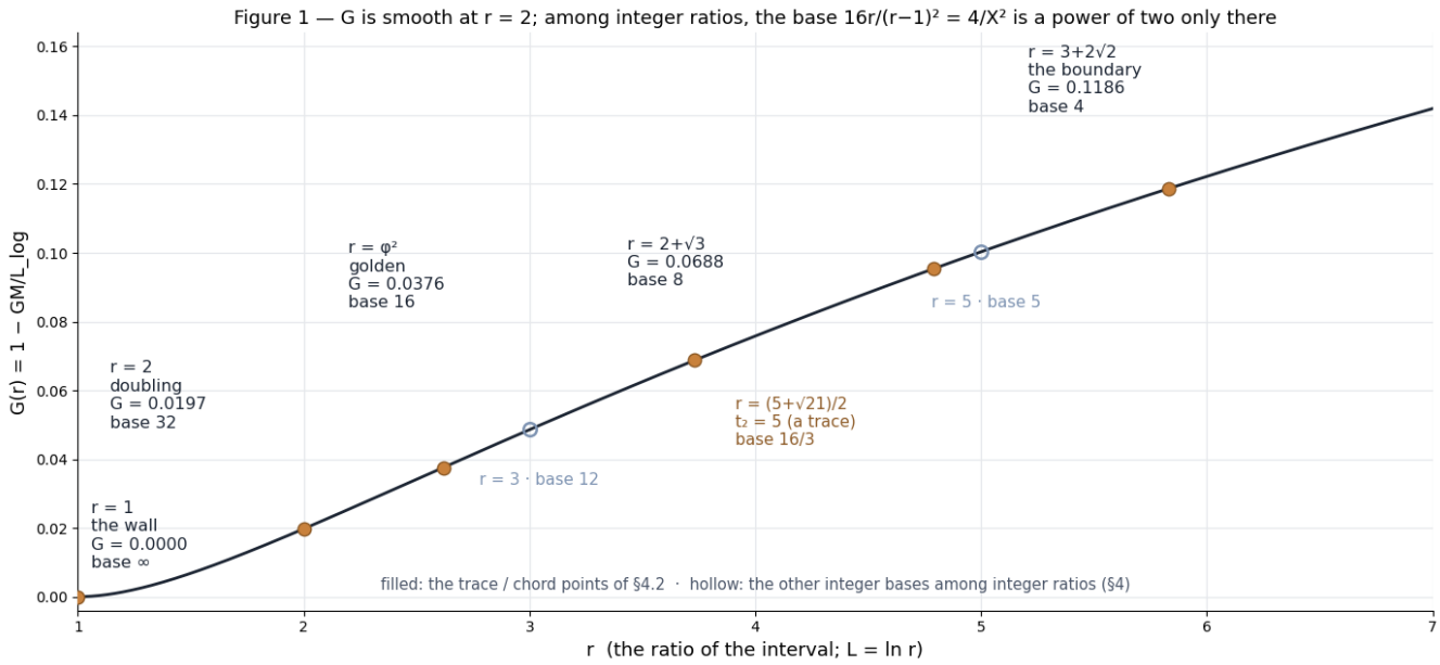
Figure 1. G(r) = 1 - GM/L_{\log} on 1 \leq r \leq 7 . Filled: the wall, the doubling interval, the golden point, 2+\sqrt{3} , (5+\sqrt{21})/2 and the boundary – the trace and chord points of §4.2 – with the series 16r/(r-1)^2 = 4/X^2 under each. Hollow: r = 3 and r = 5 , the other integer bases among integer ratios (§4). No extremum; the inflection in the coordinate r sits at 2.474..., not at 2 (§2; uniqueness in r is not claimed). The certificate's rationality ( X^2 = 1/8 ) is a line of algebra, not a feature of the curve.
