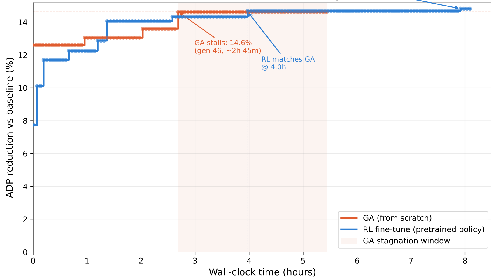
Softmax: RL fine-tune vs GA — quality over time
