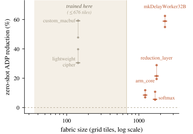
Figure 1: Zero-shot scale extrapolation. The policy is trained only on small fabrics ( \leq 676 grid tiles; shaded band). With a single zero-shot rollout per benchmark it produces ADP reductions on all six held-out benchmarks. The four larger ones lie to the right of the training band — out of distribution in size, up to 2,304 tiles ( \sim 3.4\times the area and \sim 5\times the logic of anything in the training pool) — and every one is positive across all three seeds. The two small benchmarks (custom_macbuf, lightweight_cipher; grey) are in-size controls. Dots are three seeds (7/42/123), the tick is the median, and the line spans min-max. All reductions are against the same traditional baseline.
