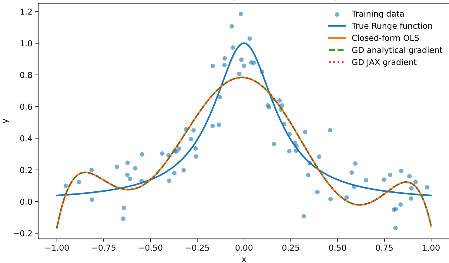
OLS: closed form and gradient descent, degree 6
