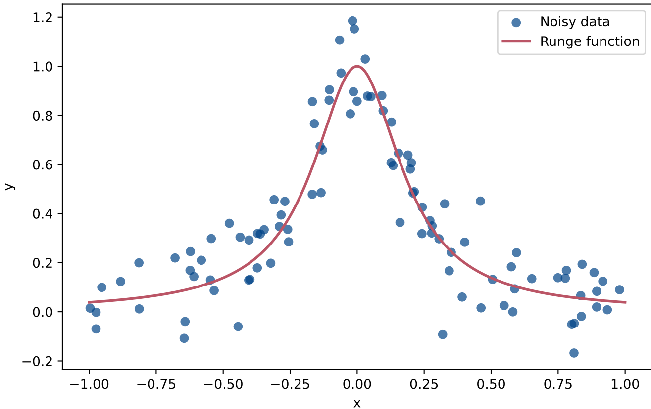
Runge function with noisy data
