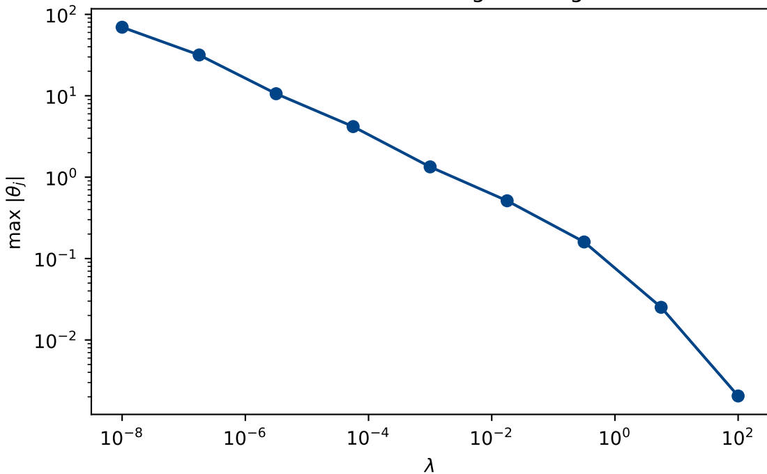
Coefficient shrinkage in Ridge
