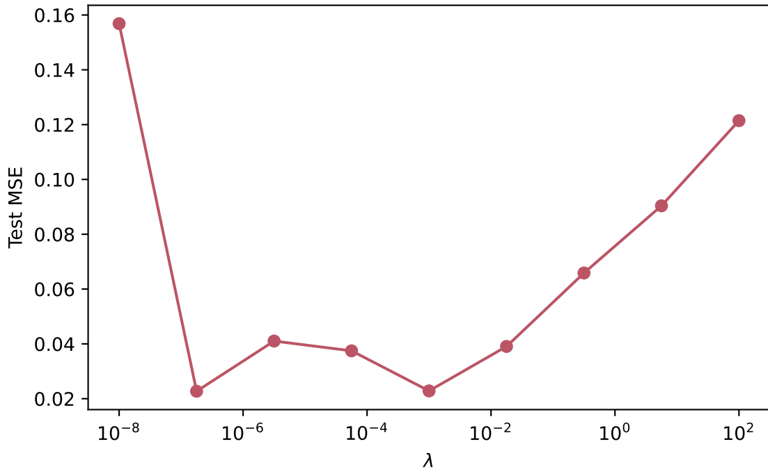
Ridge test MSE, degree = 15
