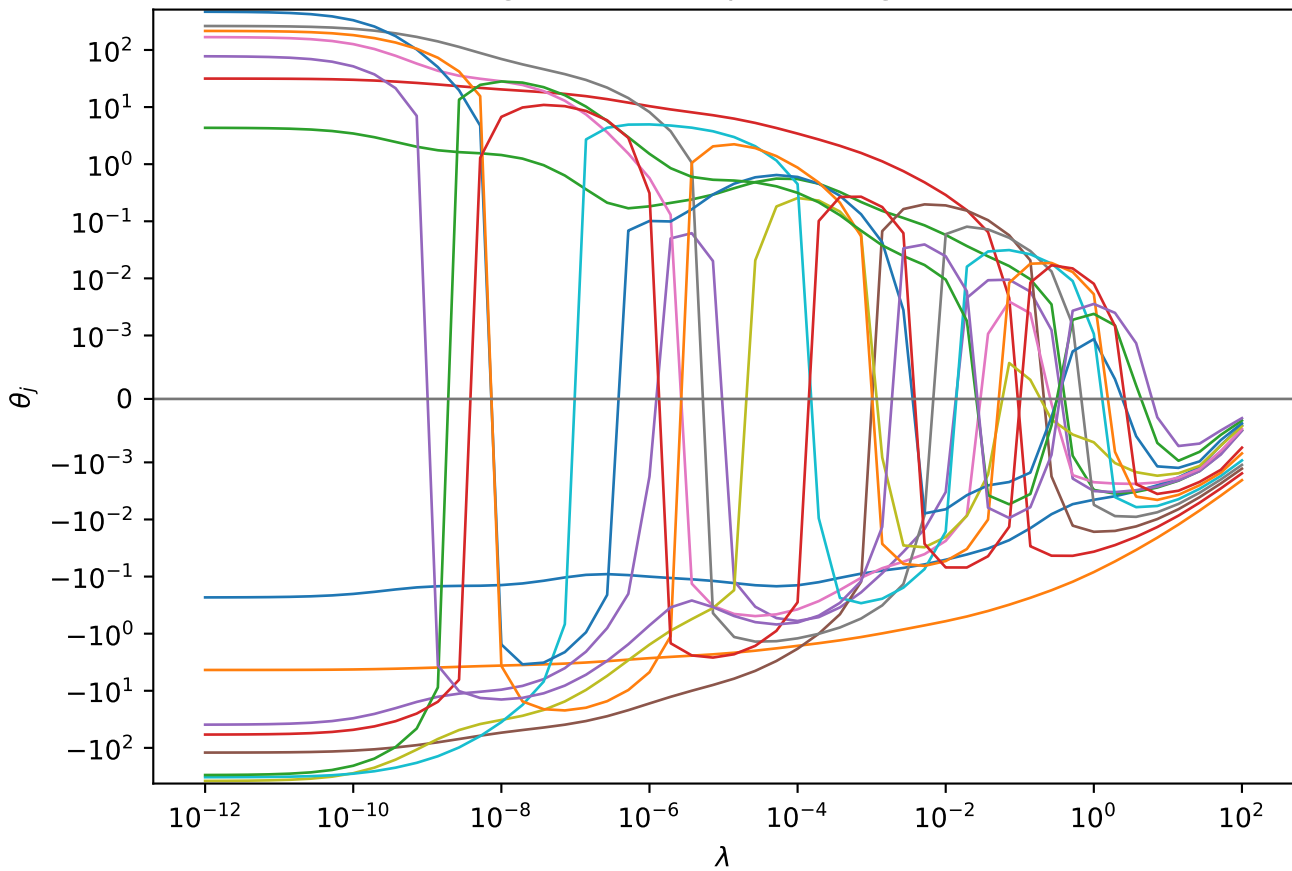
Ridge coefficient paths, degree 15
